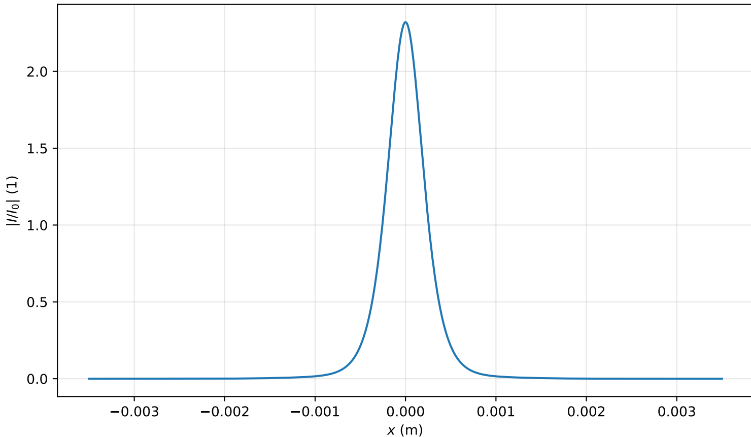
Intensity profile I(x, y = 0, z = 2.388m)/I_0 , P_{in}=1.0P_{cr} , artificial time
